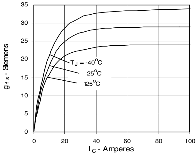
Fig. 7. Transconductance
