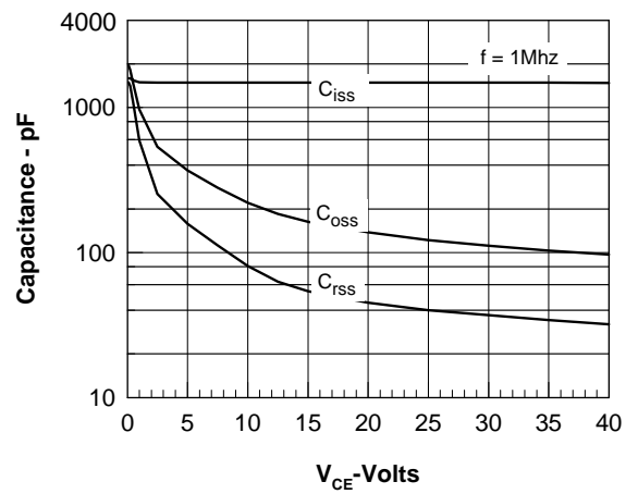
Fig. 6. Capacitance Curves
