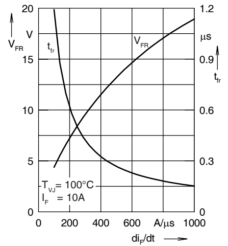
Fig. 18. Peak forward voltage V_{FR} and t_i versus di_F/dt
