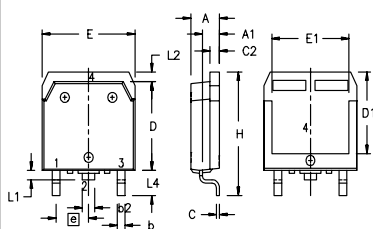
TO-268AA (D 3 PAK)
