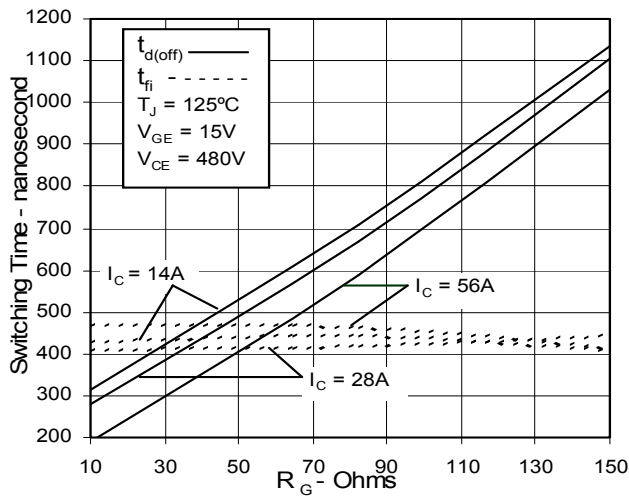
Fig. 11. Dependence of Switching Time on R_G
