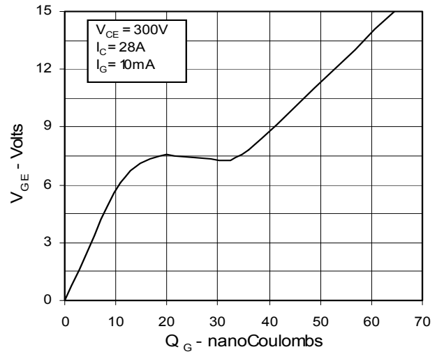
Fig. 14. Gate Charge
