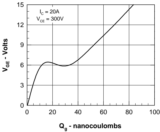
Fig. 9. Gate Charge
