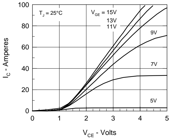
Fig. 1. Output Characteristics
