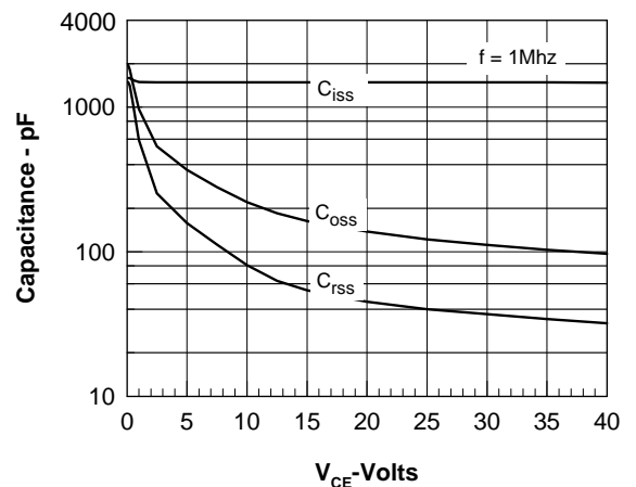
Fig. 6. Capacitance Curves
