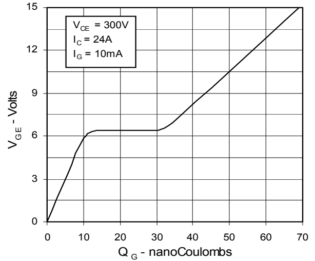
Fig. 14. Gate Charge
