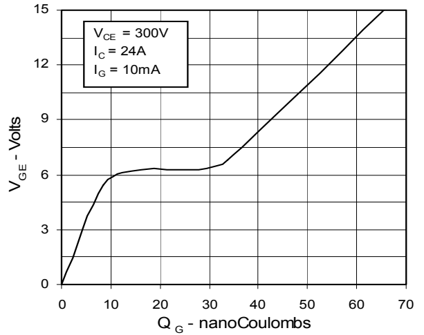
Fig. 14. Gate Charge
