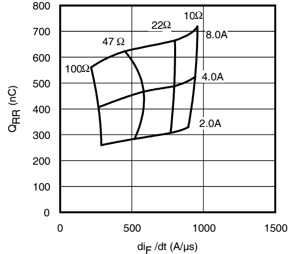
Fig. 20 - Typical Diode Q_{RR} V_{CC}=400V ; V_{GE}=15V ; T_J=175^\circ C
