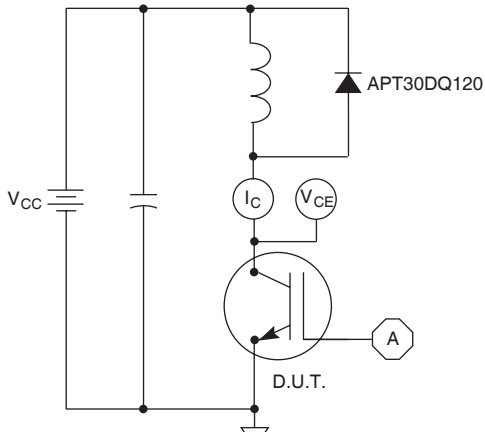
Figure 21, Inductive Switching Test Circuit
