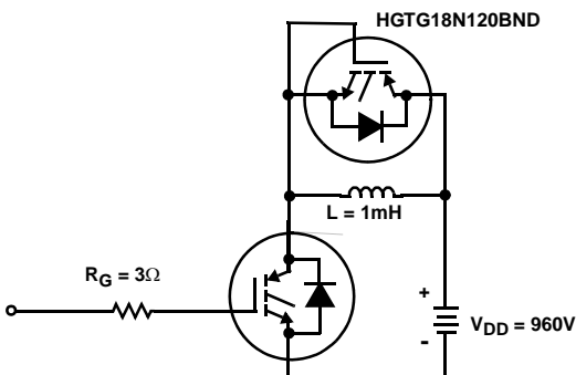
FIGURE 20. INDUCTIVE SWITCHING TEST CIRCUIT
