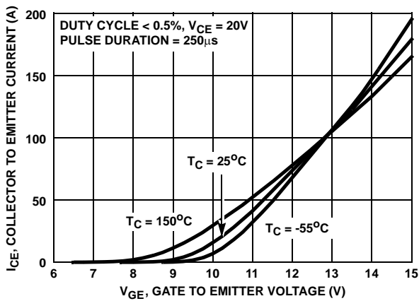
FIGURE 13. TRANSFER CHARACTERISTIC
