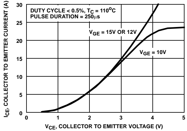
FIGURE 16. COLLECTOR TO EMITTER ON-STATE VOLTAGE
