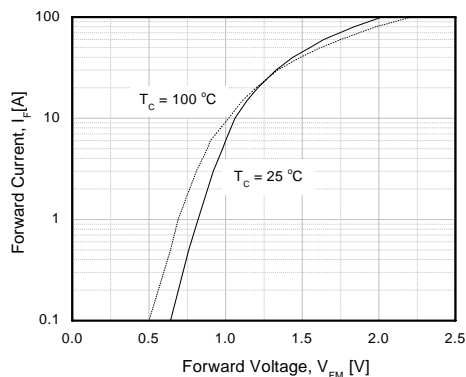
Fig 13. Forward Characteristics
