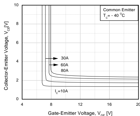
Fig 4. Saturation Voltage vs. V GE
