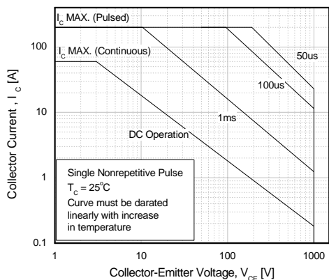
Fig 11. SOA Characteristics
