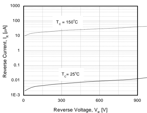
Fig 16. Reverse Current vs. Reverse Voltage
