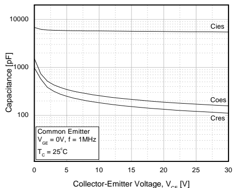
Fig 7. Capacitance Characteristics
