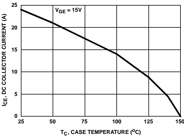
FIGURE 5. DC COLLECTOR CURRENT vs CASE TEMPERATURE
