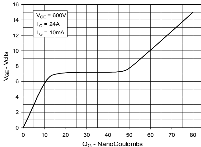
Fig. 8. Gate Charge
