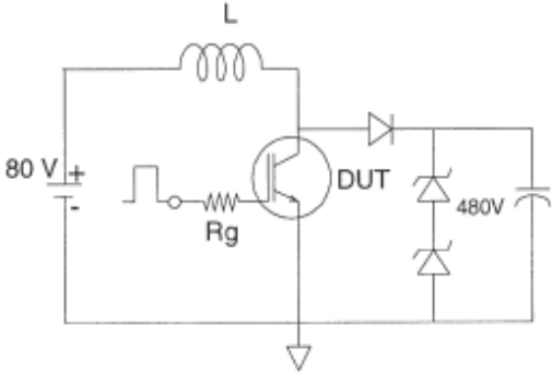
Fig.C.T.2 - RBSOA Circuit
