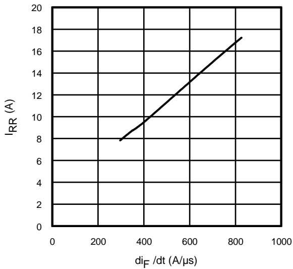
Fig. 19 - Typical Diode I RR vs. di F /dt V CC = 400V; V GE = 15V; I CE = 5.0A; T J = 150°C
