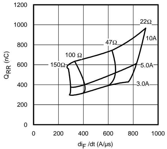
Fig. 20 - Typical Diode Q RR V CC = 400V; V GE = 15V; T J = 150°C
