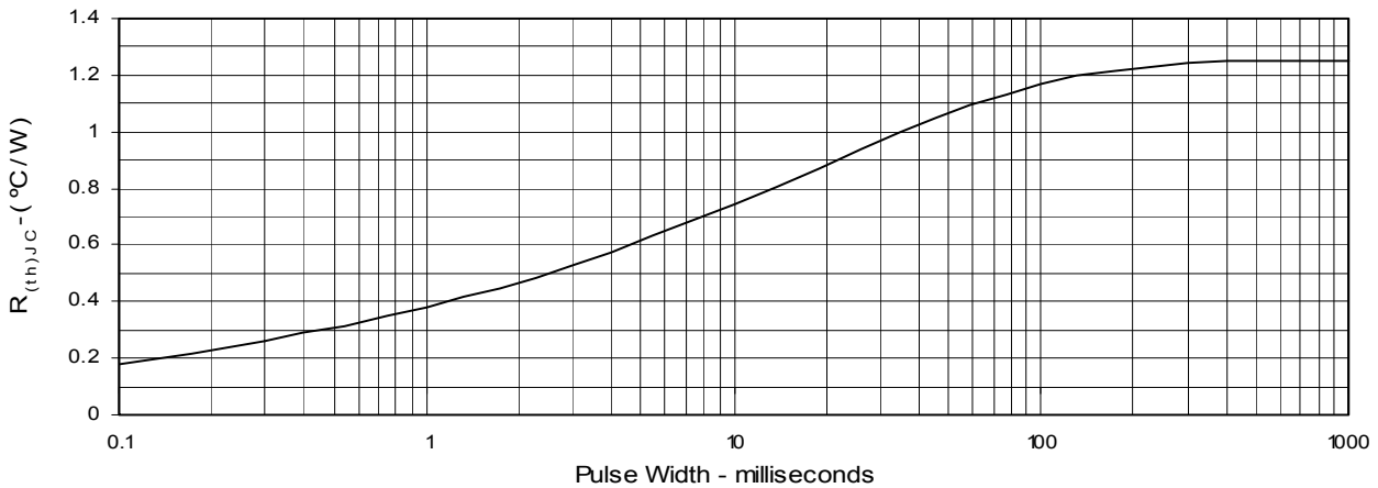
Fig. 17. Maximum Transient Thermal Resistance
