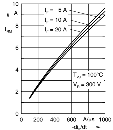
Fig. 20. Peak reverse current I_{RM} versus -di_F/dt
