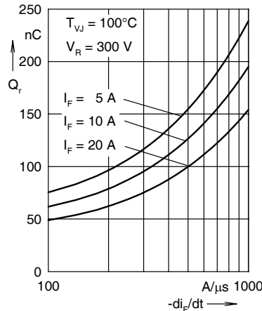
Fig. 19. Reverse recovery charge Q_r versus -di_F/dt
