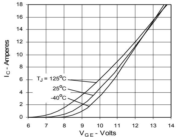
Fig. 6. Input Admittance
