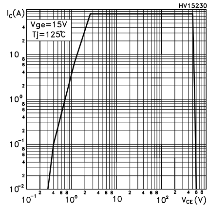
Figure 14. Turn-Off SOA
