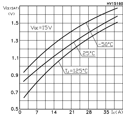
Figure 5. Collector-Emitter on Voltage vs Collector Current
