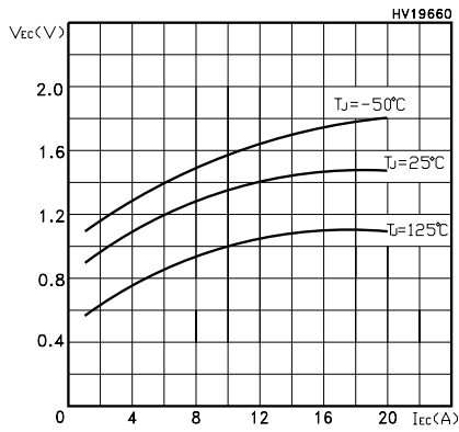
Figure 15. Emitter-Collector Diode Characteristics
