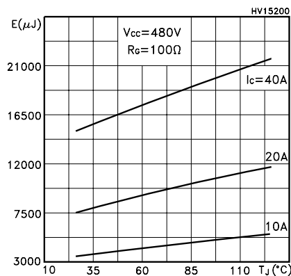
Figure 11. Switching Losses vs Temperature
