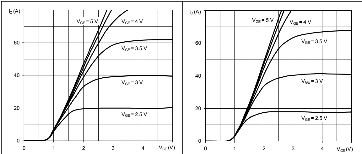
Figure 4. Output characteristics ( T_J = 25^\circ\text{C} ) Figure 5. Output characteristics ( T_J = -40^\circ\text{C} )
