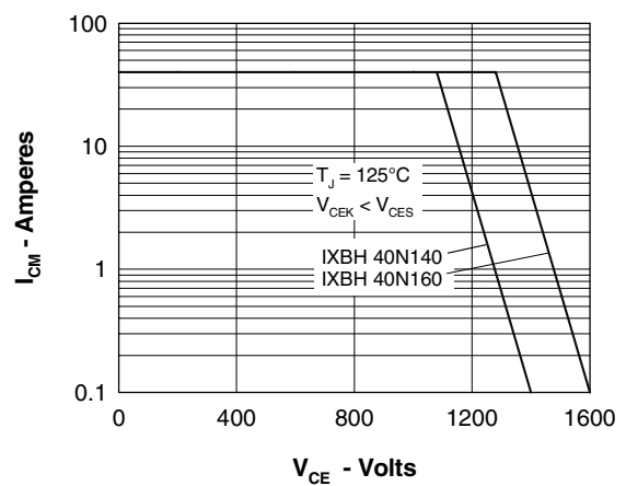
Fig. 6 Reverse Based Safe Operating Area RBSOA
