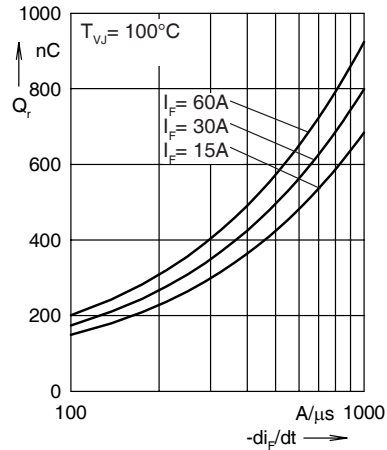
Fig. 19. Reverse recovery charge
