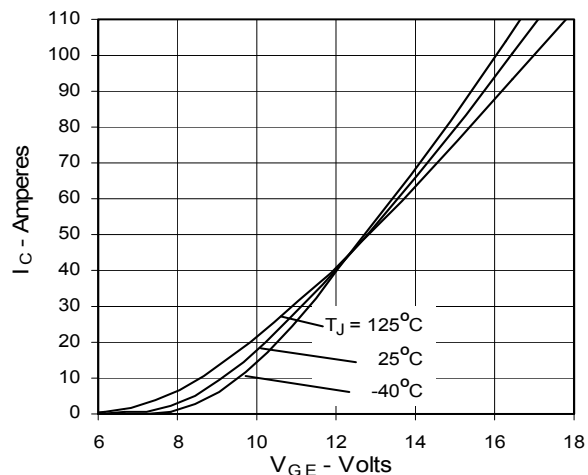
Fig. 6. Input Admittance
