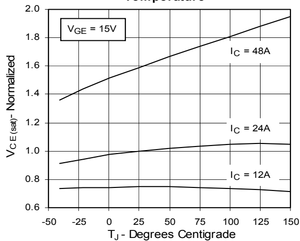
Fig. 4. Dependence of V_{CE(sat)} on Temperature
