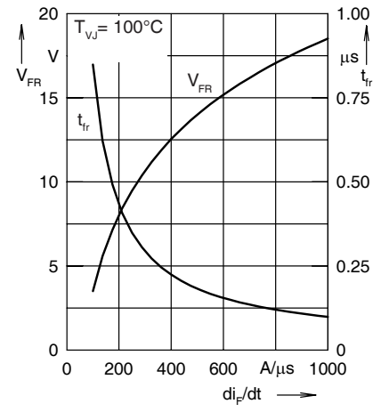
Fig. 23. Peak forward voltage V_{FR}
