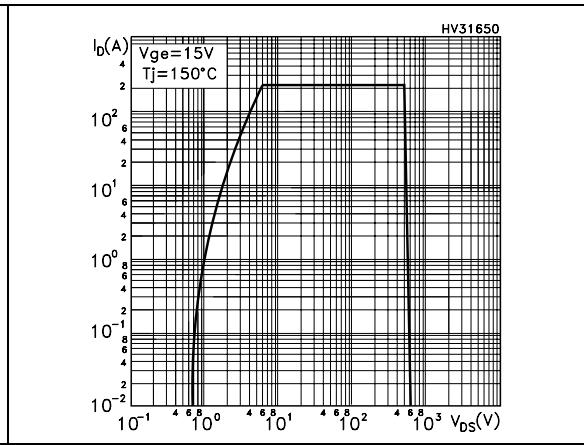
Figure 15. Turn-off SOA
