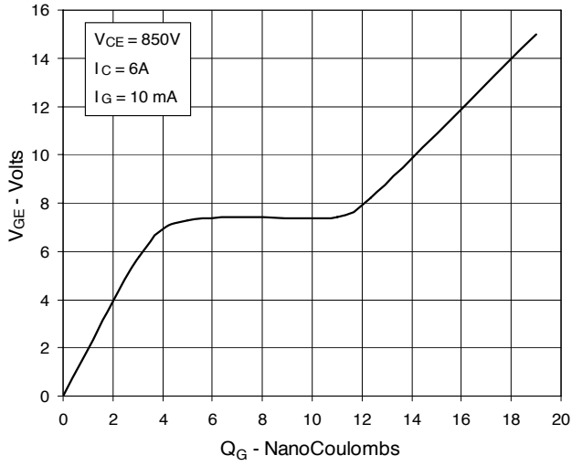
Fig. 7. Gate Charge
