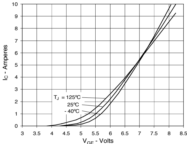
Fig. 5. Input Admittance
