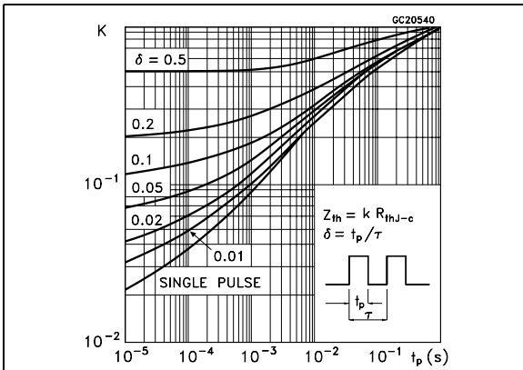
Figure 14. Thermal Impedance
