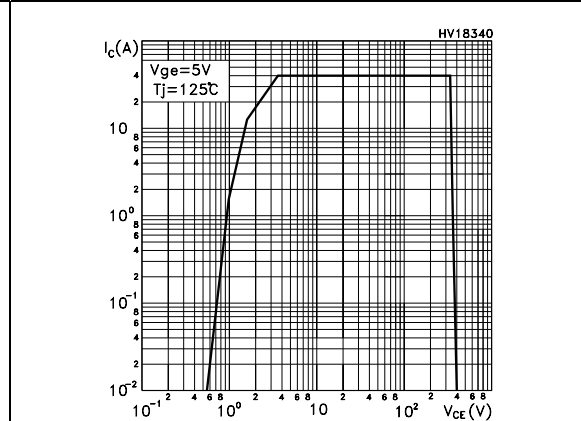
Figure 15. Turn-off SOA
