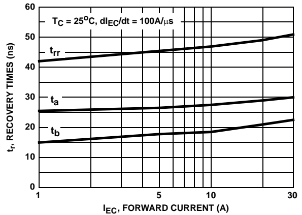
Figure 20. RECOVERY TIME vs FORWARD CURRENT
