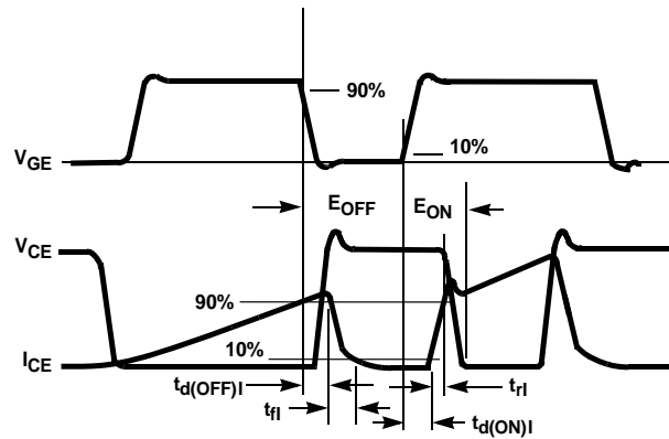
Figure 22. SWITCHING TEST WAVEFORMS
