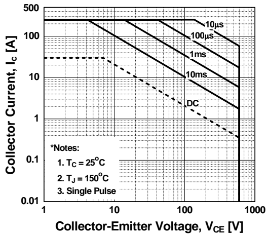
Figure 17. SOA Characteristics
