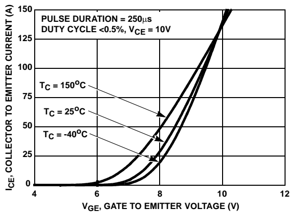
FIGURE 1. TRANSFER CHARACTERISTICS
