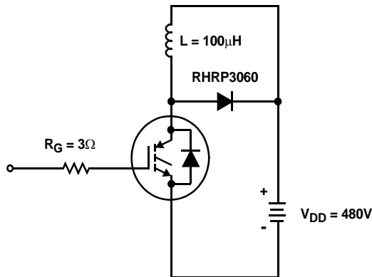
Figure 21. INDUCTIVE SWITCHING TEST CIRCUIT
