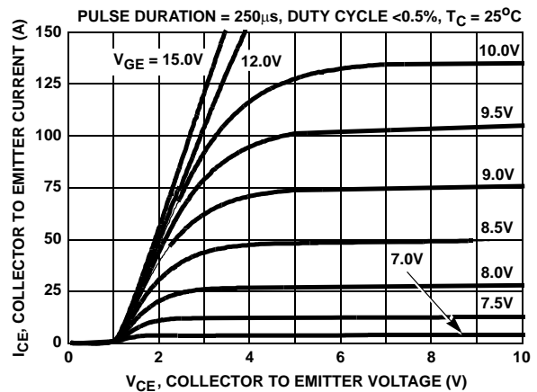
FIGURE 2. SATURATION CHARACTERISTICS
