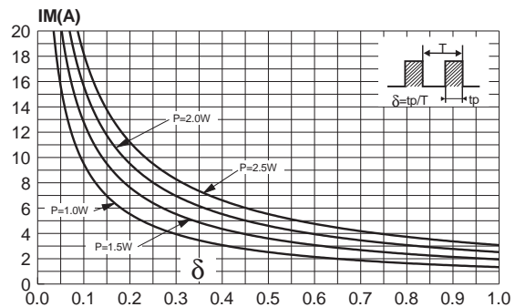
Fig. 2: Peak current versus form factor.
