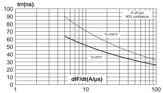
Fig. 8: Reverse recovery time versus diF/dt .
