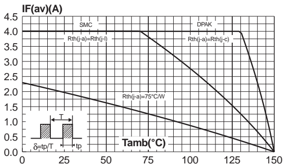
Fig. 3: Average forward current versus ambient temperature ( \delta=0.5 ).
