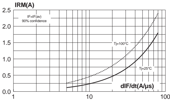
Fig. 7: Reverse recovery current versus diF/dt .
