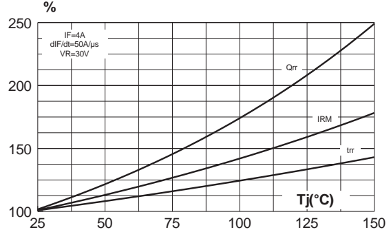
Fig. 10: Dynamic parameters versus junction temperature.
