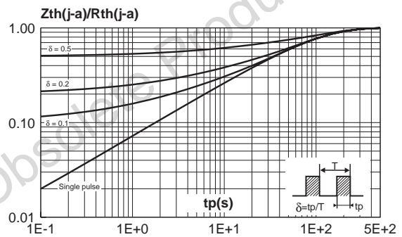
Fig. 4: Variation of thermal impedance junction to ambient versus pulse duration (recommended pad layout, epoxy FR4, \epsilon(\text{Cu}) = 35\mu\text{m} ).
