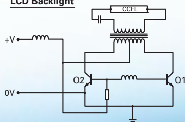
Figure 4. Resonant converter for LCD backlight
