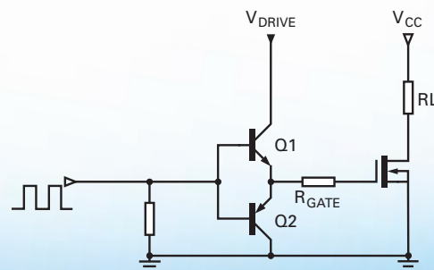
Figure 3. Totem-pole driver stage for power MOSFET
