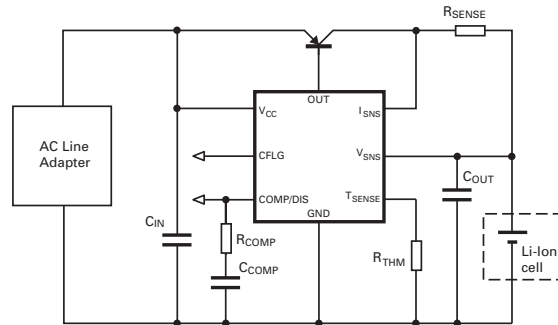
Figure 2. A typical linear charger circuit
