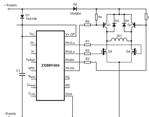
Figure 5. Single-phase fan motor circuit
