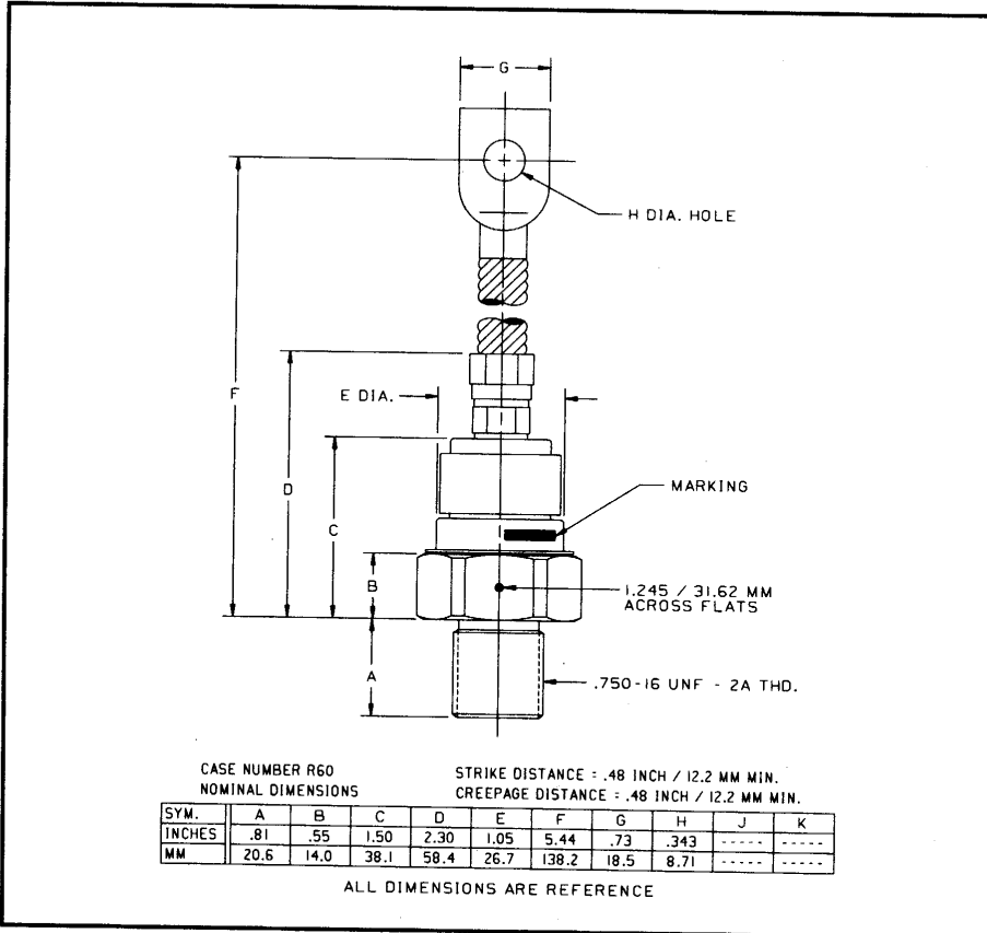
R602__25/R603__25 (Outline Drawing)
