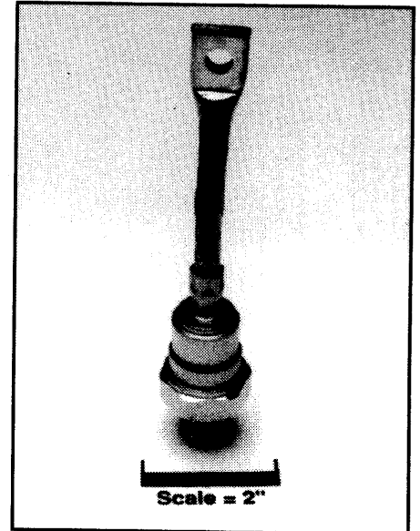
R602__25/R603__25 Fast Recovery Rectifier 250 Amperes Average, 1600 Volts
