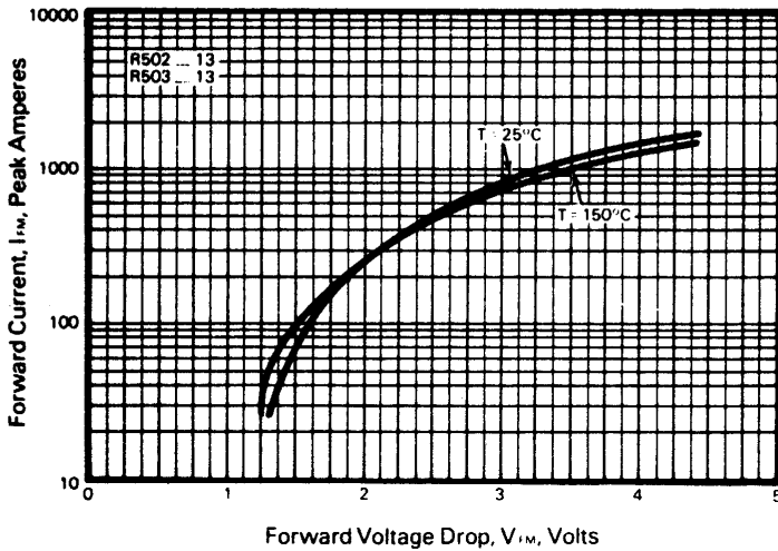
Forward Current Vs. Forward Voltage Drop
