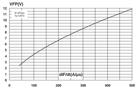
Fig. 9: Transient peak forward voltage versus dI_F/dt (90% confidence).
