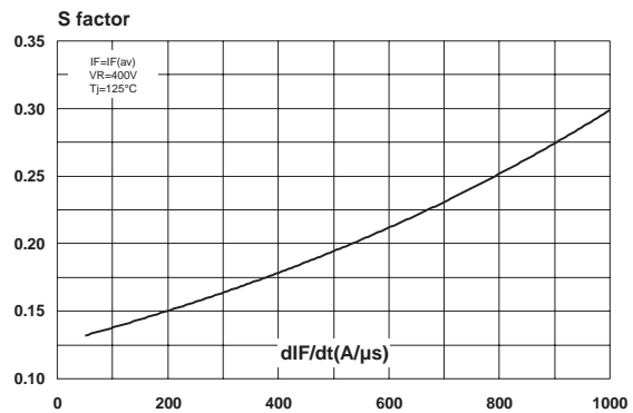
Fig. 7: Softness factor versus dI_F/dt (typical values).
