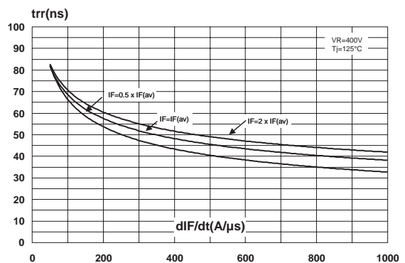
Fig. 5: Reverse recovery time versus dI_F/dt (90% confidence).
