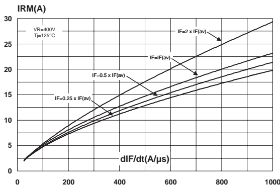
Fig. 4: Peak reverse recovery current versus dI_F/dt (90% confidence).
