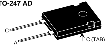
TO-247 AD
