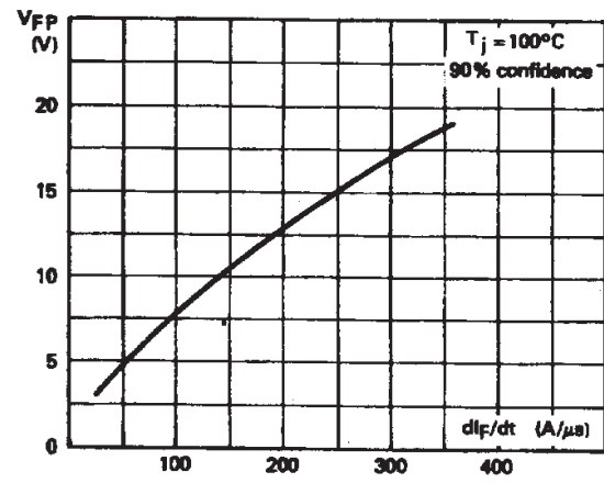
Fig.10 : Peak forward voltage versus di_F/dt .
