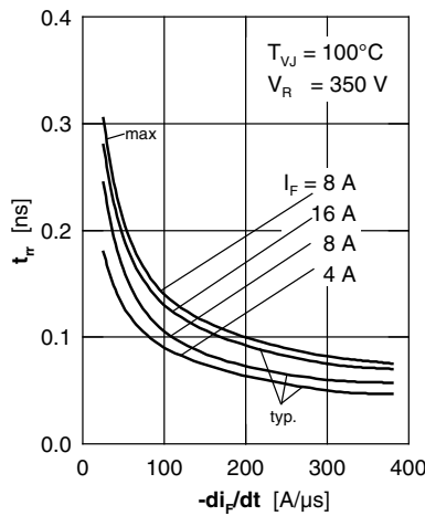
Fig. 5 Recovery time versus -di_F/dt
