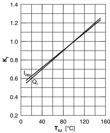
Fig. 4 Dynamic parameters versus junction temperature
