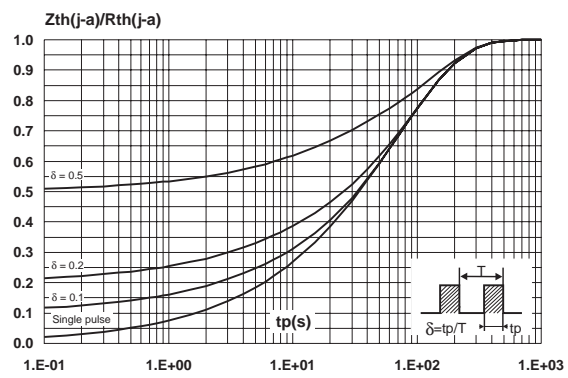
Fig. 4: Relative variation of thermal impedance junction ambient versus pulse duration (printed circuit board epoxy FR4, LLeads = 10mm).
