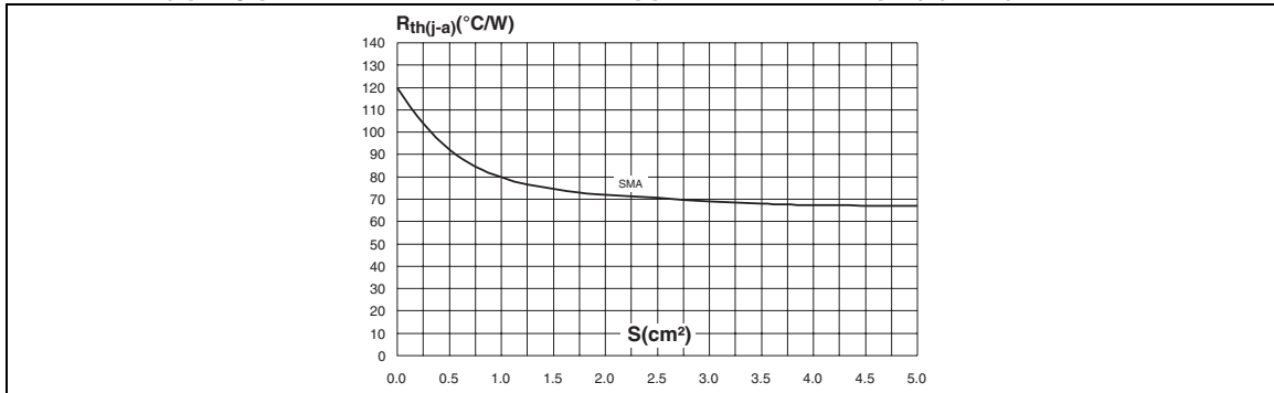
Figure 7. Thermal resistance junction to ambient versus copper surface under each lead (epoxy printed circuit board FR4, copper thickness: 35 \mu m) (SMA)
