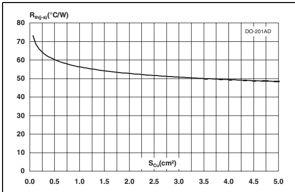
Figure 15. Thermal resistance junction to ambient versus copper surface under each lead, DO-201AD (epoxy FR4, copper thickness = 35 μm)
