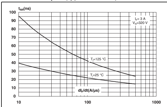
Figure 9. Reverse recovery time versus di_F/dt (typical values)
