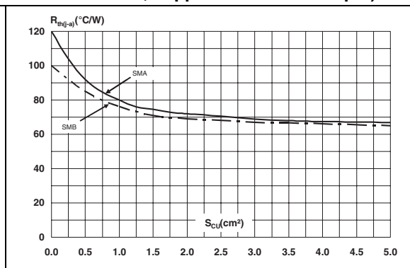
Figure 16. Thermal resistance junction to ambient versus copper surface under each lead, SMA, SMB, (epoxy FR4, copper thickness = 35 \mu\text{m} )
