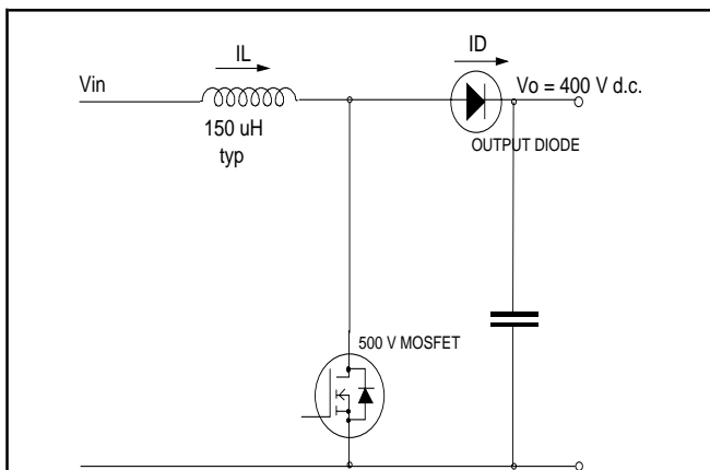
Fig. 1. Typical application, output rectifier in boost converter power factor correction circuit. Continuous conduction, mode where the transistor turns on whilst forward current is still flowing in the diode.
