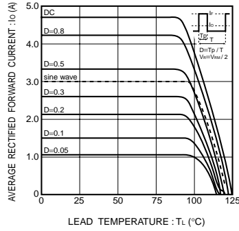
Fig.5 Derating curve (Io - Tl) (When mounted on alumina PCBs)
