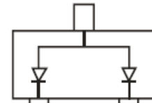
BAS40-06T Marking: 46
