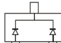
BAS40-05T Marking: 45
