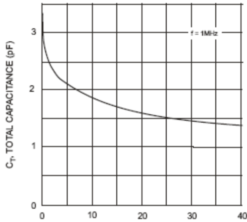
Fig. 3 Typical Capacitance
