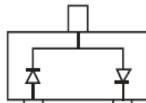
BAS40-04T Marking: 44
