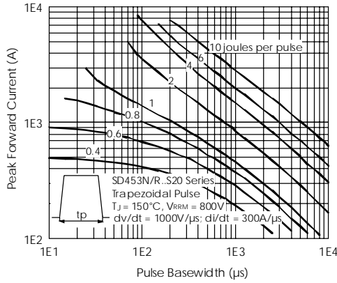
Fig. 26 - Maximum Total Energy Loss Per Pulse Characteristics
