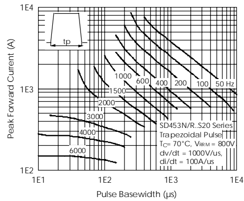
Fig. 29 - Frequency Characteristics
