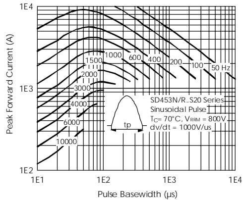
Fig. 25 - Frequency Characteristics
