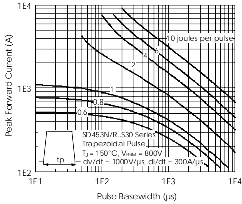
Fig. 32 - Maximum Total Energy Loss Per Pulse Characteristics
