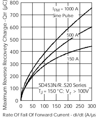
Fig. 19 - Recovery Charge Characteristics
