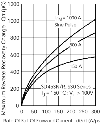
Fig. 22 - Recovery Charge Characteristics
