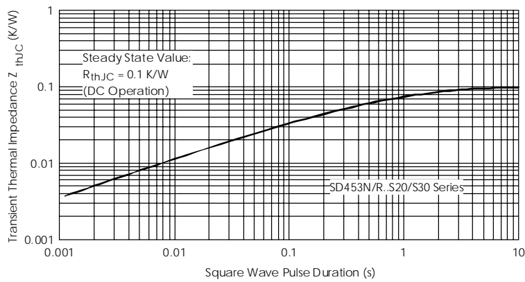
Fig. 15 - Thermal Impedance Z_{thJC} Characteristic
