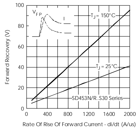
Fig. 17 - Typical Forward Recovery Characteristics
