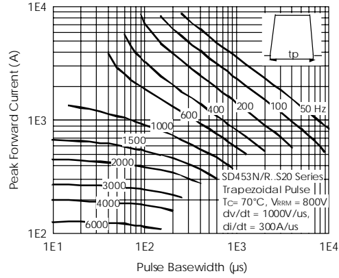
Fig. 27 - Frequency Characteristics
