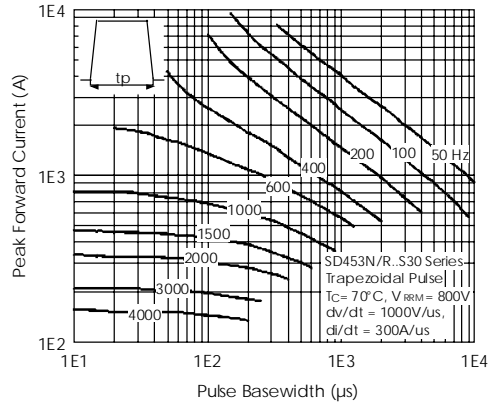
Fig. 33 - Frequency Characteristics
