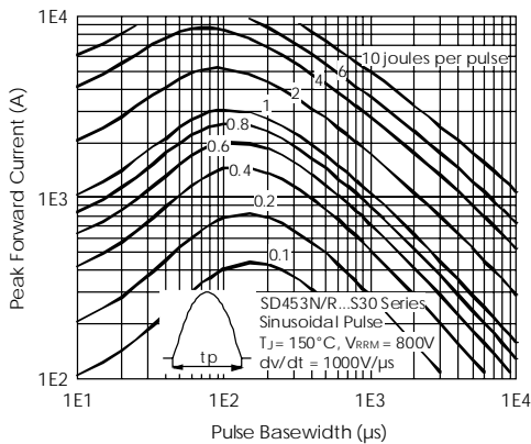
Fig. 30 - Maximum Total Energy Loss Per Pulse Characteristics
