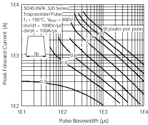
Fig. 28 - Maximum Total Energy Loss Per Pulse Characteristics
