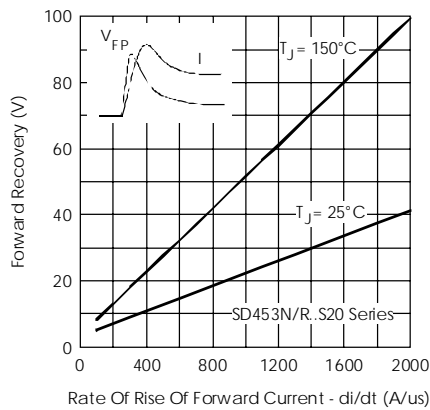
Fig. 16 - Typical Forward Recovery Characteristics
