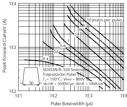
Fig. 34 - Maximum Total Energy Loss Per Pulse Characteristics
