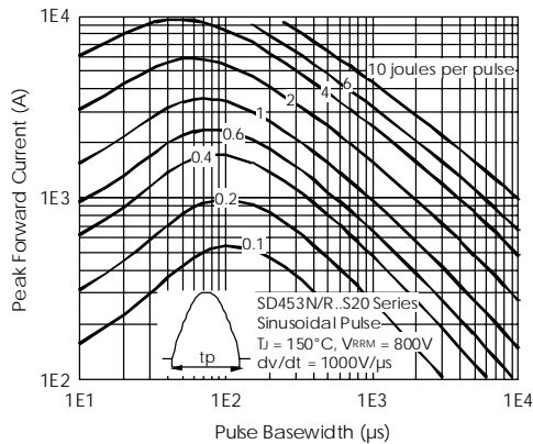
Fig. 24 - Maximum Total Energy Loss Per Pulse Characteristics
