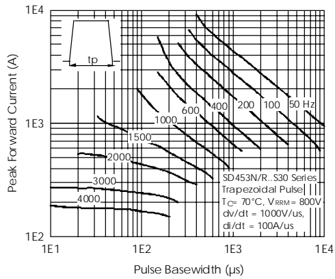
Fig. 35 - Frequency Characteristics
