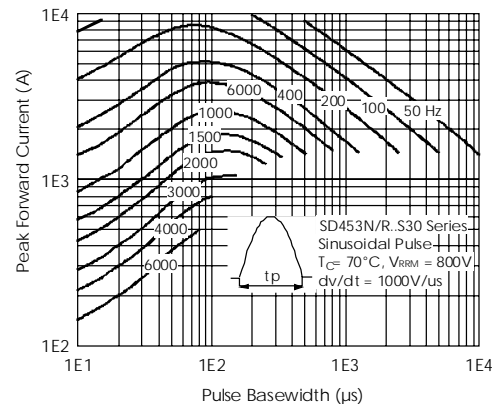
Fig. 31 - Frequency Characteristics
