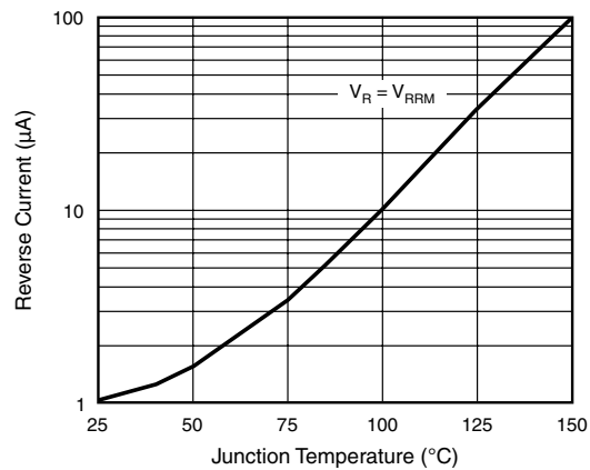
Figure 2. Reverse Current vs. Junction Temperature
