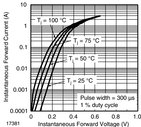
Figure 3. Typical Instantaneous Forward Characteristics - SL02
