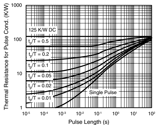
Figure 8. Thermal Response
