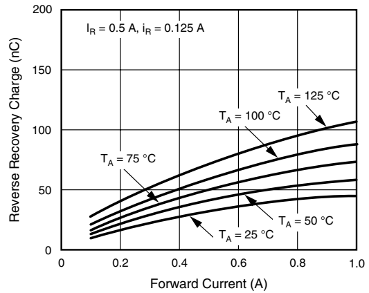
Figure 7. Reverse Recovery Charge vs. Forward Current
