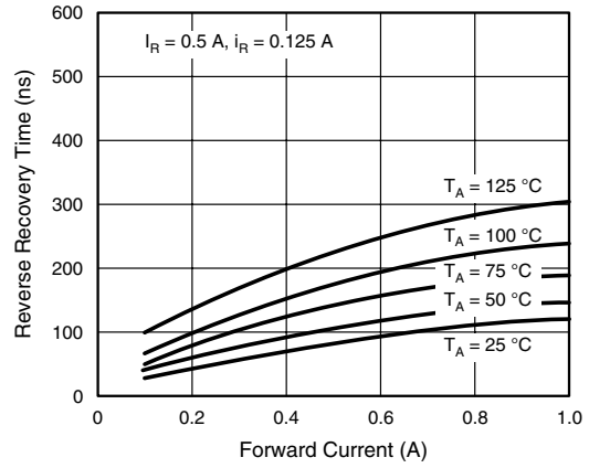
Figure 6. Reverse Recovery Time vs. Forward Current
