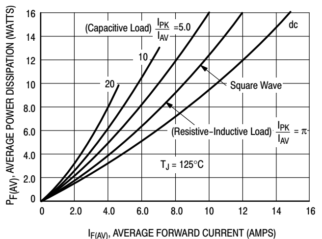
Figure 15. Power Dissipation
