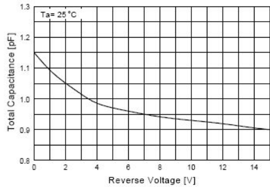
Figure 8. Total Capacitance
