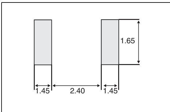
Figure 15: SMA Foot Print Dimensions (in millimeters)
