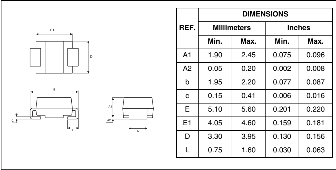
Figure 16: SMB Package Mechanical Data
