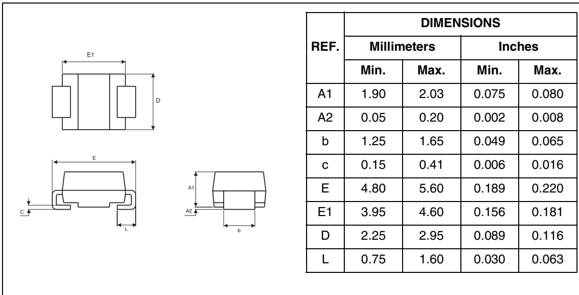
Figure 14: SMA Package Mechanical Data
