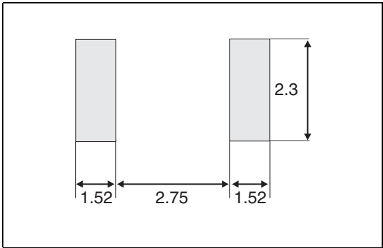
Figure 17: SMB Foot Print Dimensions (in millimeters)
