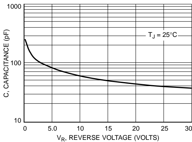
Figure 7. Capacitance
